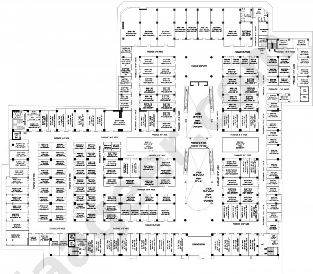
FIRST FLOOR PLAN SCALE: 1/16" = 1'-0" NO OF SHOPS = 183
